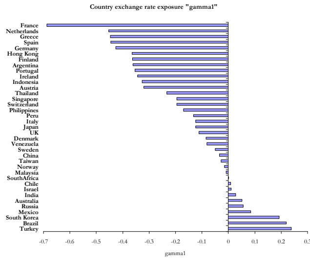
Figure 3: Gamma1 estimations
