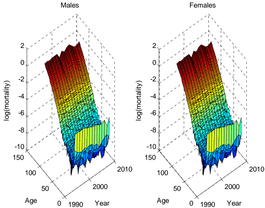
Figure 2: Logarithm of Raw Central Death Rates in China, 1994-2008
