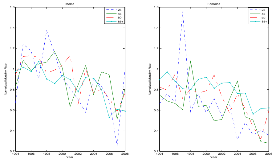
Figure 1: Normalized Death Rate for Selected Age Groups
