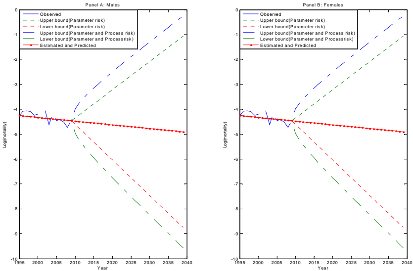
Figure 5: Prediction of Log Mortality Rate at 60 with Parameter Risk
