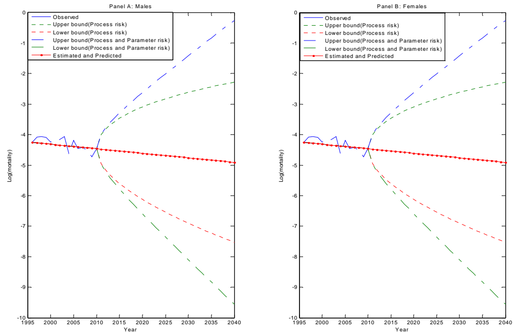
Figure 6: Prediction of Log Mortality Rate at 60 with Process Risk
