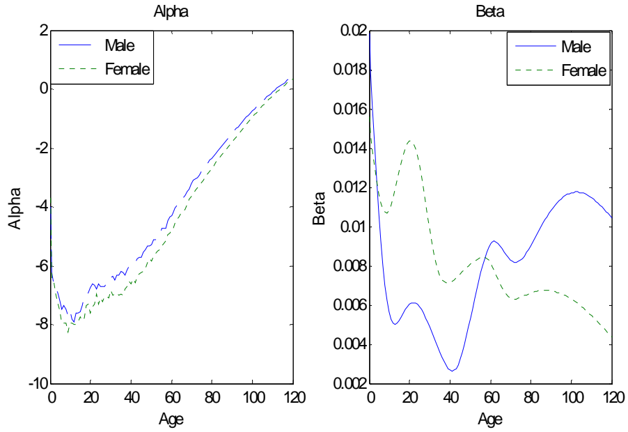
Figure 3: Estimated \alpha_x and \beta_x
